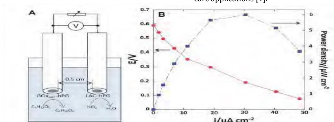
Figure1. Scheme of the enzymatic biofuel cell set up. B: Polarisation and power density curve of the GOx ads hPG and LAC-hPG biofuel cell. The power and the current density refer to the total superficial surface area of the electrodes used (0.03 cm 2 ).
