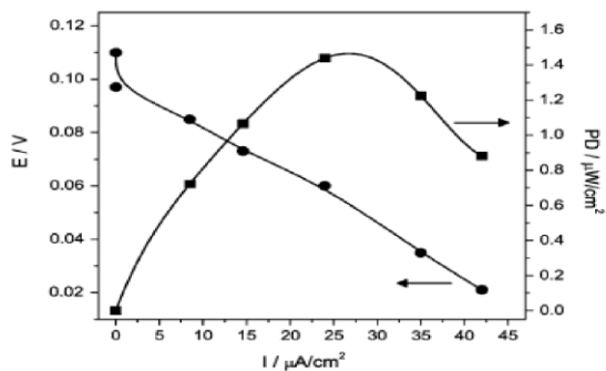
Figure 3. Polarization and power density (PD) curves acquired at 30C using SPEEK as electrolyte membrane and mediator less N-GOx-MWCNTs-f on CC as bio anode. Fuel 1 M glucose solution.
