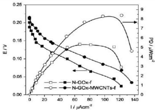
Figure 2. Polarization and power density (PD) curves acquired at 30 C using N-GOx-f and N-GOx-MWCNTs-f on CC as bioanodes. Methylene blue was used as redox mediator in bioanode chamber. Fuel 1 M glucose solution
