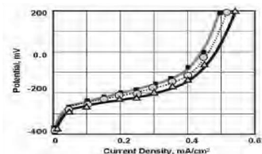
Figure 4. Polarization curves of three TP/MWNTs/PEI, GOx, Nafion electrodes. 20 mM phosphate buffer, pH 6.9, 0.1M KCl, 20 mM glucose 20 C. 0.1 cm 2 electrodes.
