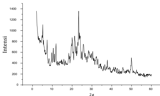
Figure 5: XRD of FLR-1:1
