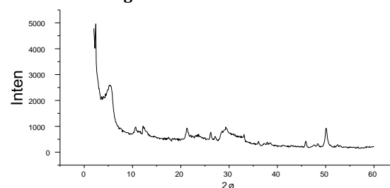
Figure 3: XRD of Florite
