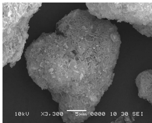
Figure 9: SEM of Florite
