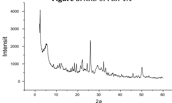
Figure 6: XRD of FLR-1:1
