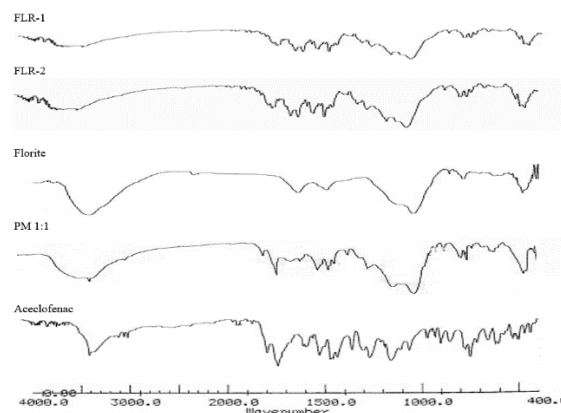
Figure 1: IR Spectra
