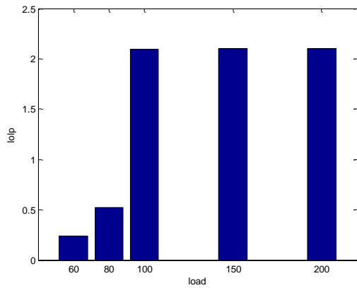
Figure 2. Effect of increasing the peak load on the LOLP.
