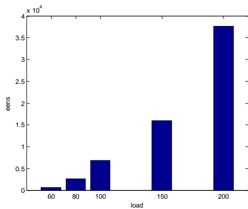
Figure 4. Effect of increasing the peak load on the EENS
