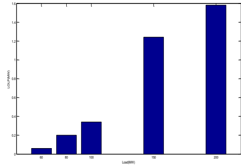
Figure 5. effect of increasing the peak load LOLP integrating wind farm.
