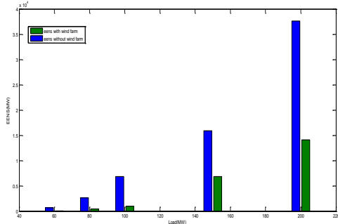
Figure 10. Comparison of peak load on EENS increases in the presence and absence of wind plant.
