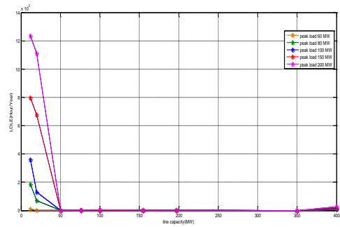
Figure 11. Variation in system LOLE with line capacity of the wind farm.
