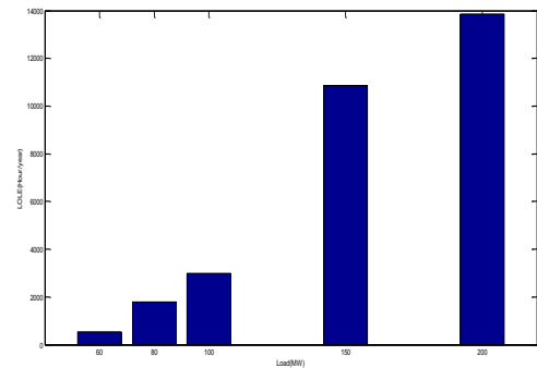
Figure 6. Effect of increasing the peak load on the LOLE integrating wind farm.
