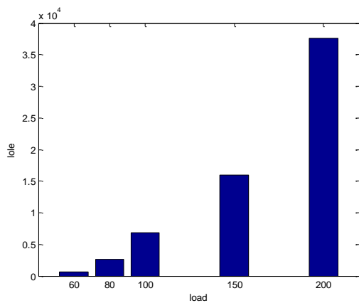
Figure 3. Effect of increasing the peak load on the LOLE.
