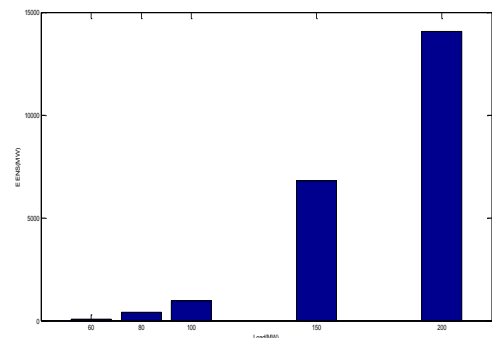
Figure 7. Effect of increasing the peak load on the EENS integrating wind farm.
