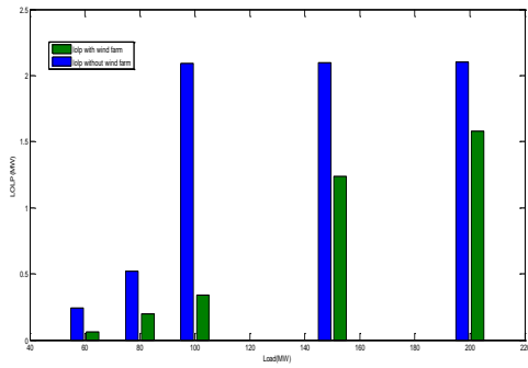
Figure 8. Comparison of the effect of increasing the peak load on the LOLP in the presence and absence of wind plant.
