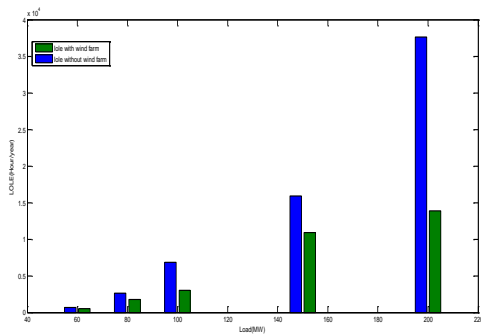
Figure 9. Comparison of the effect of increasing the peak load on the LOLE in the presence and absence of wind plant.
