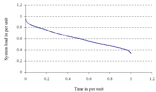
Figure 1. Model of Load Curve EEHC.
