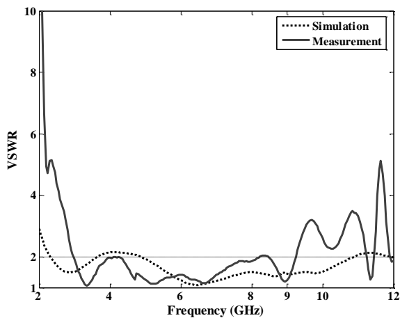
Figure 2. The VSWR response of the proposed directional UWB antenna with dimensions given in Table I.
