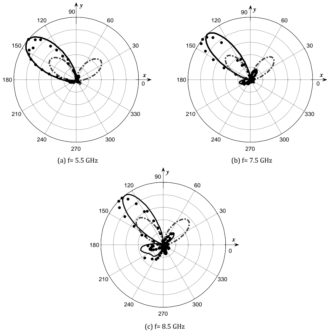
Figure 4. Simulated radiation pattern of the proposed directional UWB antenna (solid line) and of the conventional circular ring UWB monopole (dash-dotted line) in the x-y plane at three different spot frequencies. The measured radiation pattern of the proposed antenna represented with black circles. Results are reported in linear scale.
