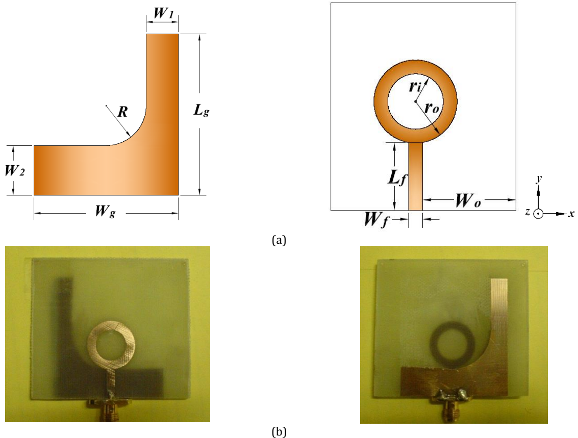
Figure 1. Geometry of proposed directional UWB antenna. (a) Schematic and, (b) photograph of fabricated antenna.
