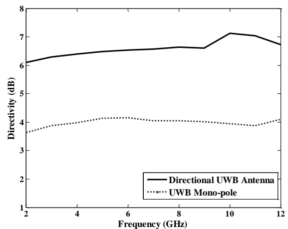
Figure 3. Antenna directivity of conventional UWB monopole (dotted line) and proposed directional UWB antenna.
