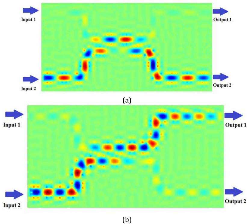
Figure 7. Electric field distributions of the directional coupler with square lattice of rods for normalized frequency of (a) f = 0.3 and (b) f = 0.32 .
