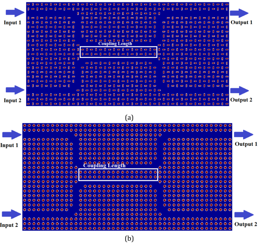
Figure 4. The proposed structures of optical photonic crystals wavelength selective devices based on directional couplers with two new geometric forms.
