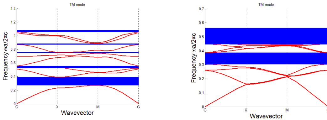
Figure 3. Photonic band structure of two-dimensional periodic photonic crystal in TM mode.
