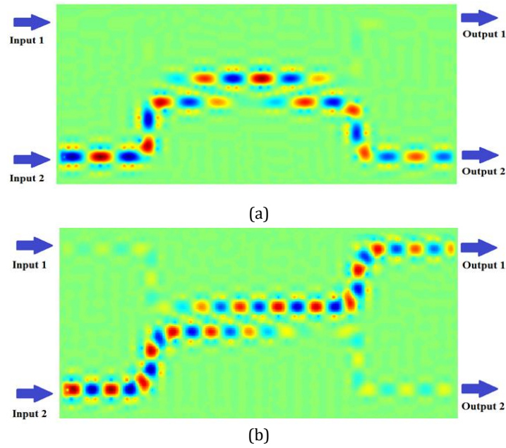
Figure 6. Electric field distributions of the directional coupler with square lattice of rods for normalized frequency of (a) f = 0.3115 and (b) f = 0.3364 .
